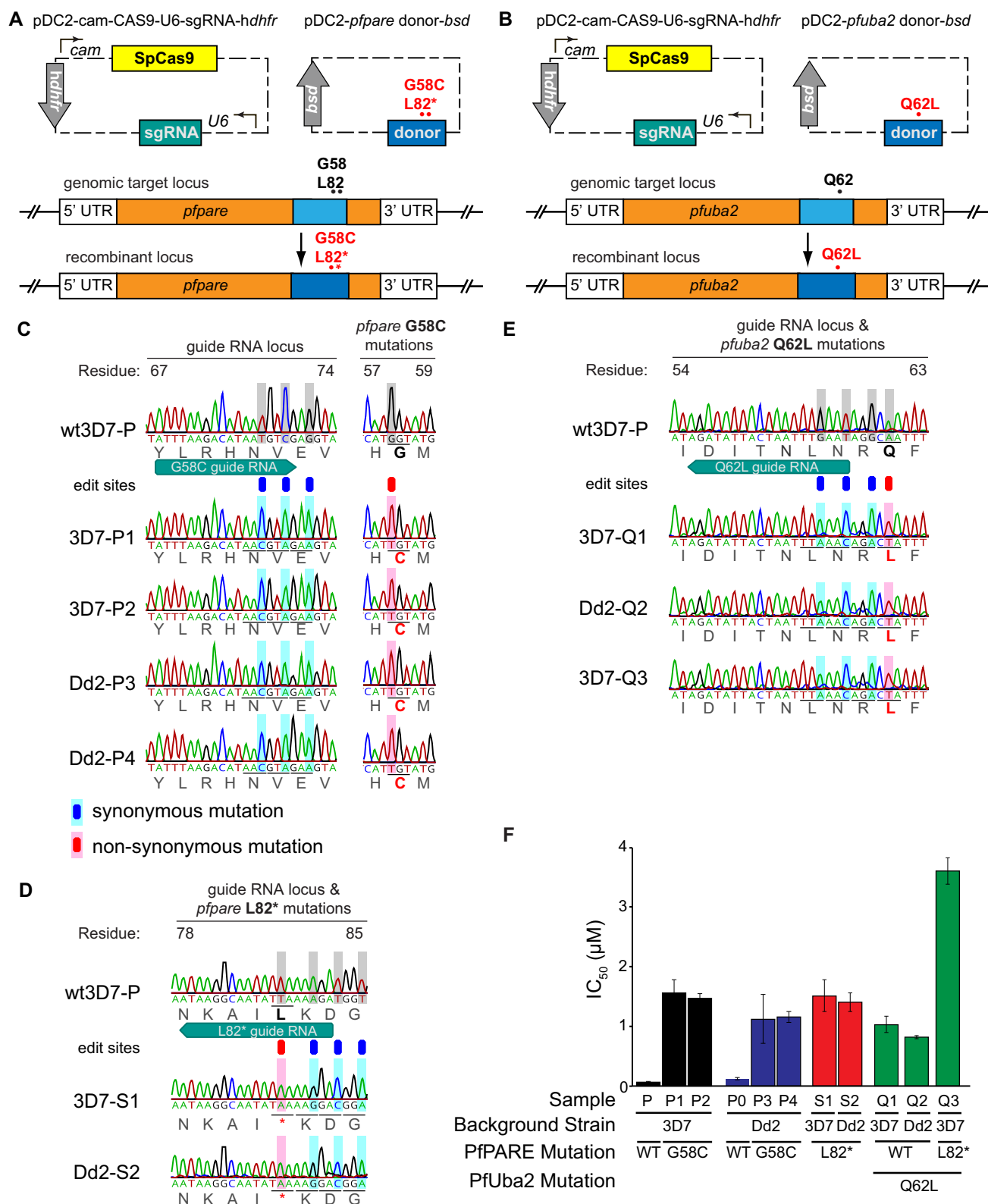
FIG 4 (A and B) CRISPR-Cas9-mediated gene editing. Dd2 and 3D7 parental parasites were transfected with a plasmid encoding the sgRNA, Cas9 nuclease, and human dihydrofolate reductase ( dhfr ) as a selectable marker, and another plasmid encoding a donor sequence containing PfPARE G58C or L82* (A) and PfUba2 Q62L (B). (C to E) Electropherograms showing unmodified and genome-edited parasites. Gray boxes highlight nucleotides that differ from wild-type parasites. PfPARE and PfUBA2 single-letter amino acid substitutions and/or stop mutations are indicated in red. (F) Susceptibility to AN13762 of the parental (WT) lines and genetically modified lines. Lines P and P0 are WT strains. P1, P3, and Q1 were cultured under 150 nM AN13762 drug pressure, and lines P2, P4, Q2, Q3, S1, and S2 were selected with WR29910 and blasticidin. Bars represent mean IC 50 values, and error bars are the standard deviations of the results from 3 independent experiments, each performed in triplicate. UTR, untranslated region.
